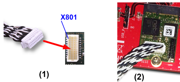
Figure 5: Connecting cable to basic card, example CIFX M223090AE
