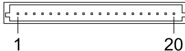
Figure 7: Cable connector Ethernet X1; 1x20 pins, AIFX-V2-RE
