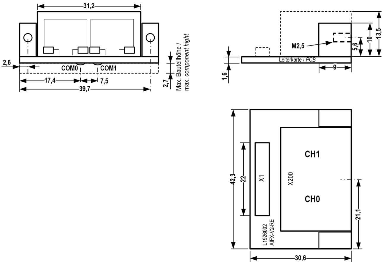
Figure 9: Dimensions AIFX-V2-RE (revision 2)
