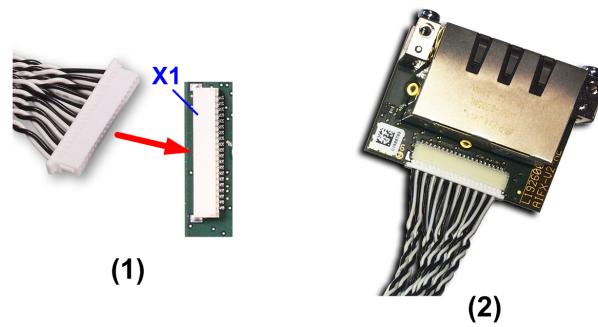
Figure 4: Connecting cable to the detached network interface Ethernet (AIFX-V2-RE)
